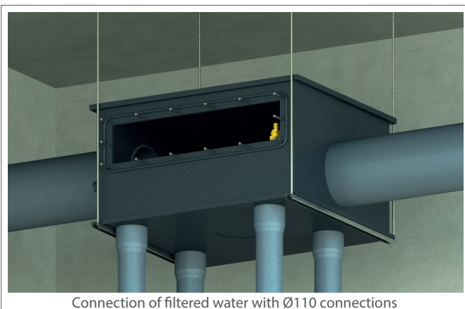
Connection of filtered water with \text{Ø}110 connections
